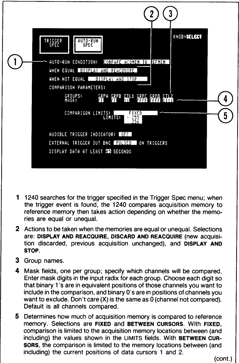
Figure 4-6. Menu display for the COMPARE ACQMEM TO REFMEM Auto-Run condition. The selected data in acquisition memory must be identical to the corresponding data in reference memory, including time relationships between two-timebase data, for the memories to be considered equal.
