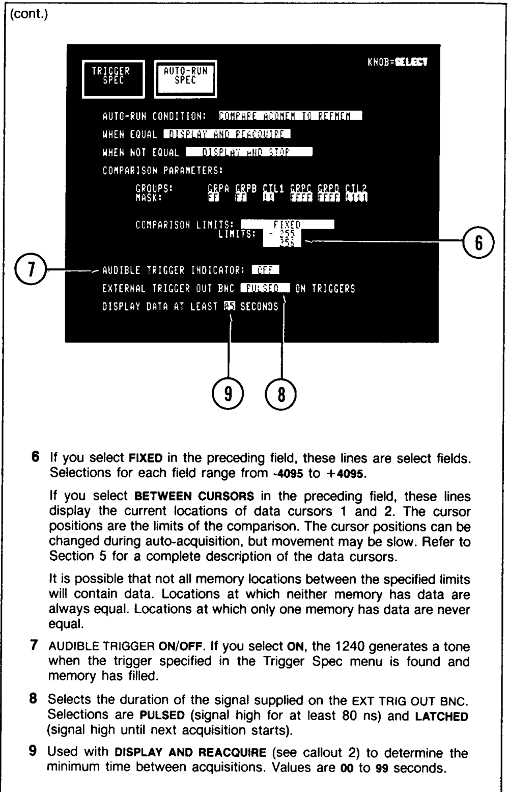
Figure 4-6. Menu display for the COMPARE ACQMEM TO REFMEM Auto-Run condition (cont.).
