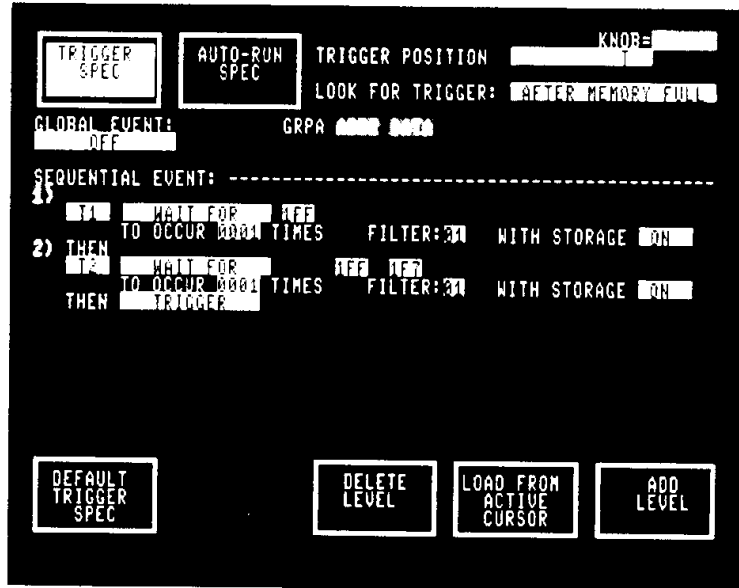
Figure 2-9. Setup of the Trigger Spec menu for the second example.
