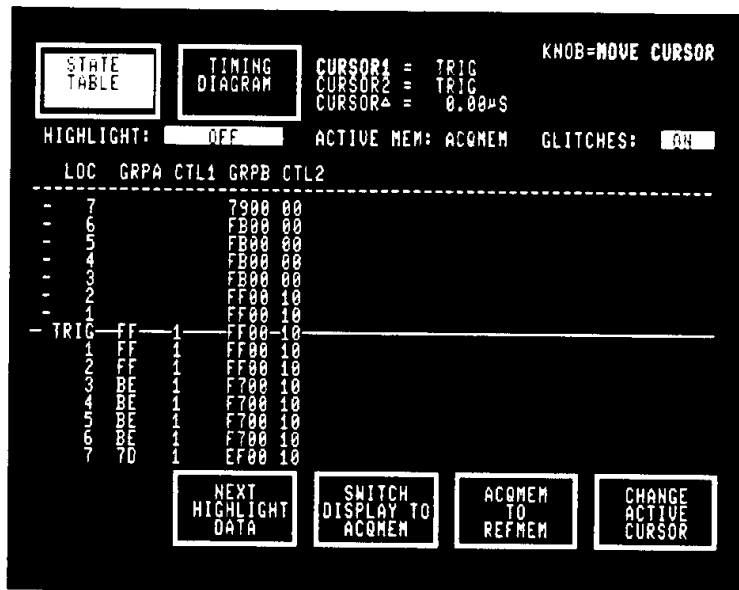
Figure 2-3. Data acquired at 20 ns ASYNC after triggering on FF in the TPG pattern.
